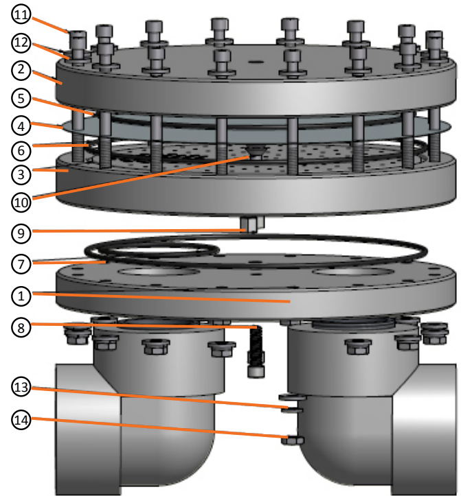
Exploded View of Equilibar BD
